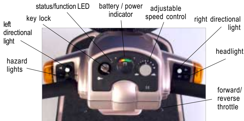
(Overview of tiller control panel)
